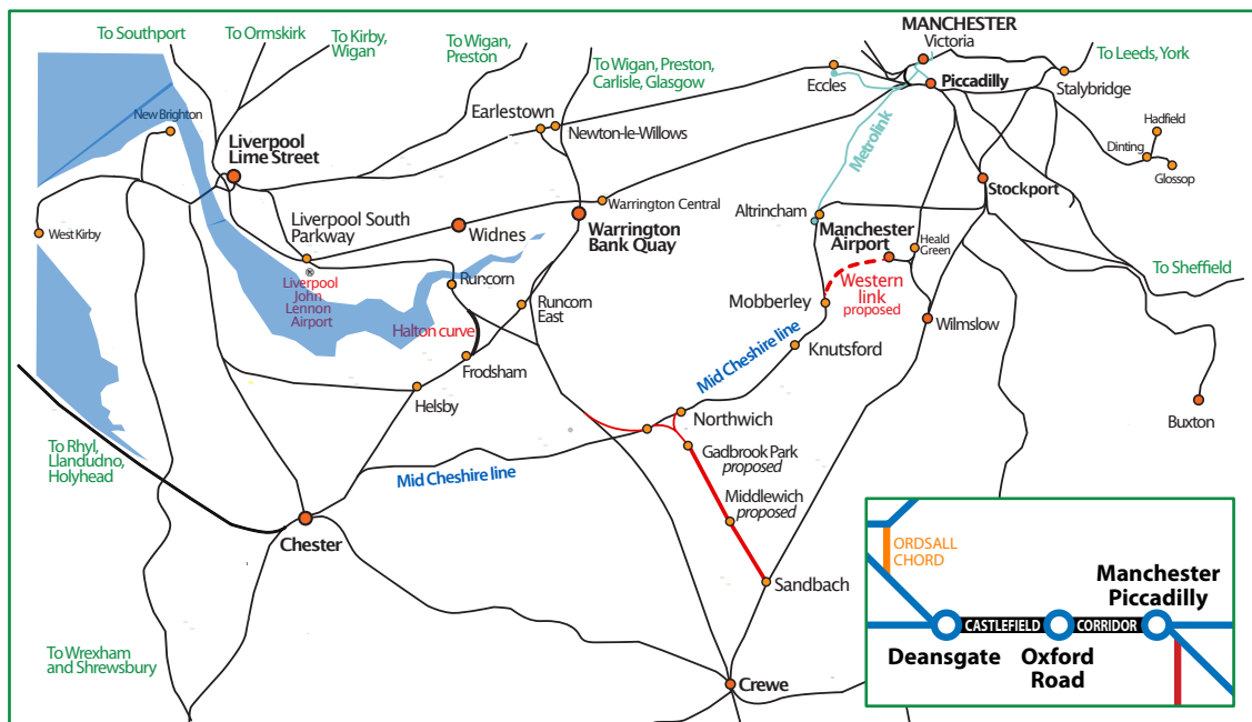
How the Manchester airport western link fits into the complex rail network south of Manchester and, inset, the overcrowded Castlefield corridor which the airport western link would help to relieve
